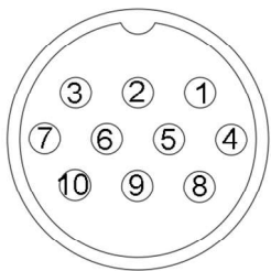
Plug viewed from solder side
